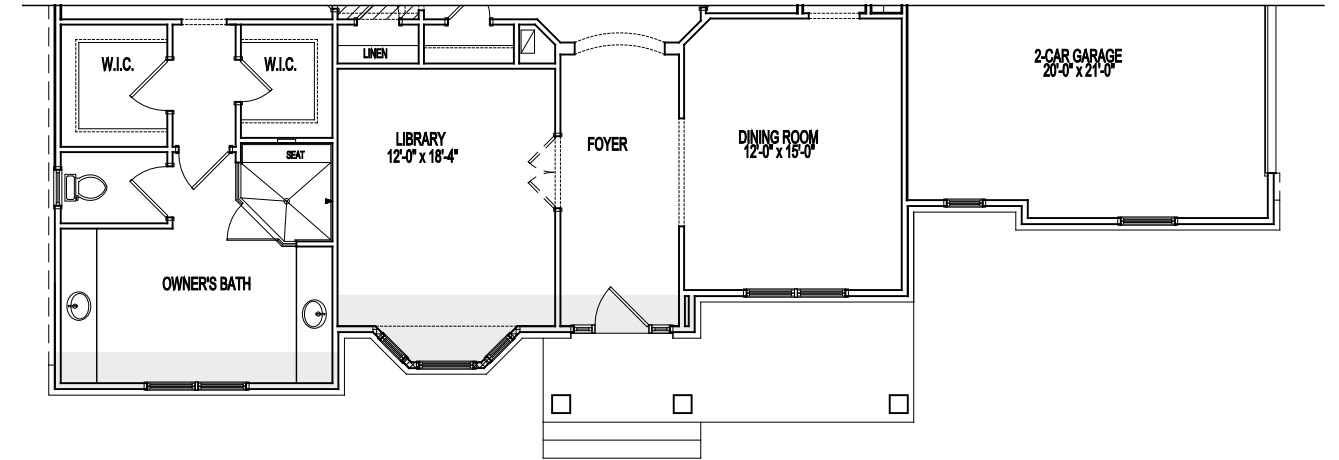
PARTIAL FIRST FLOOR PLAN ELEVATION 10B
