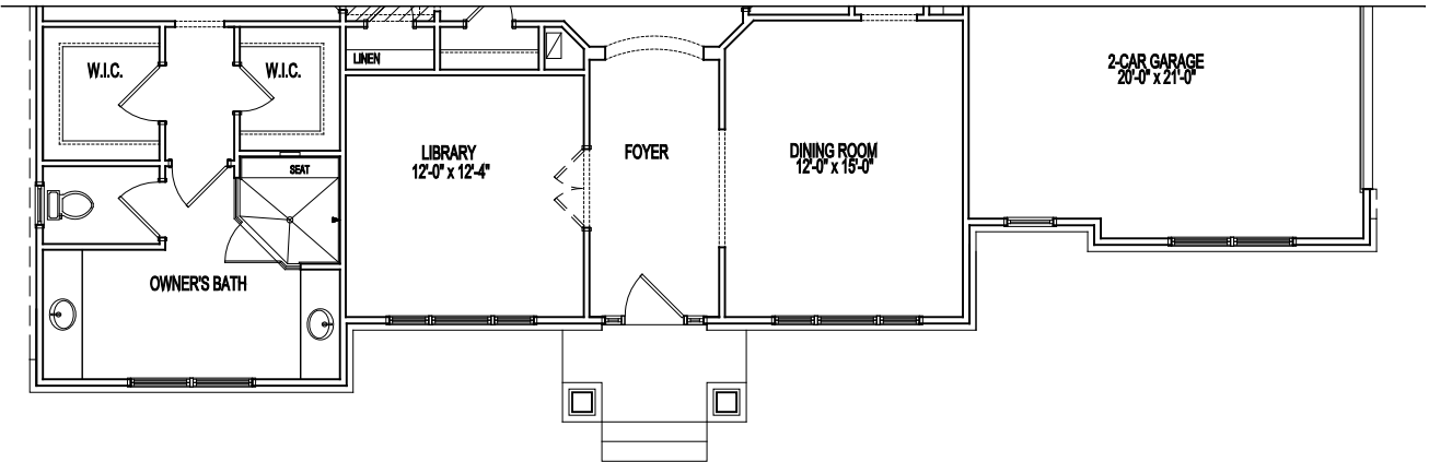
PARTIAL FIRST FLOOR PLAN ELEVATION 6A
