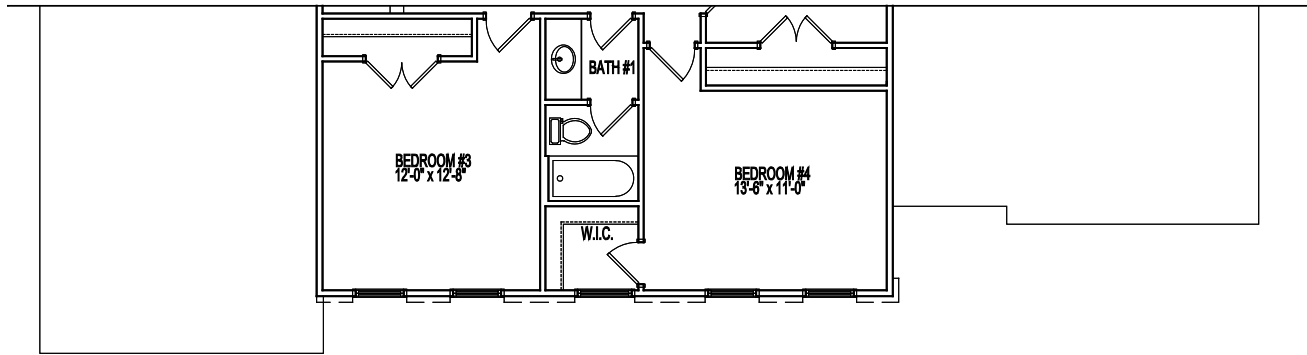
PARTIAL SECOND FLOOR PLAN ELEVATION 6A
