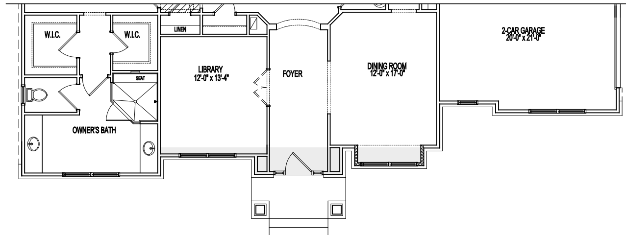
PARTIAL FIRST FLOOR PLAN ELEVATION 11A
