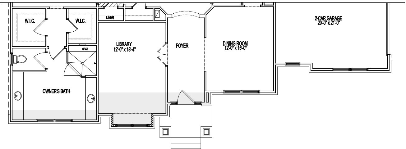
PARTIAL FIRST FLOOR PLAN ELEVATION 5A
