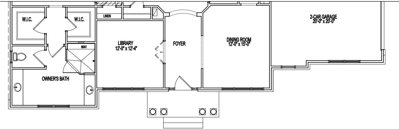
PARTIAL FIRST FLOOR PLAN
