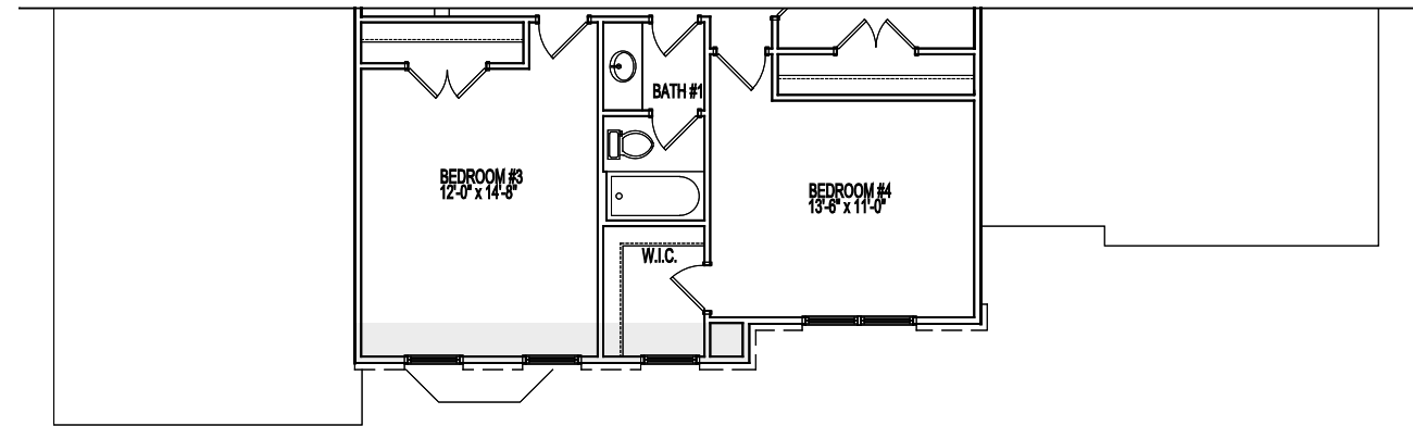
PARTIAL FIRST FLOOR PLAN ELEVATION 10B
