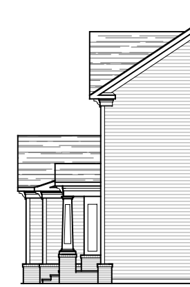
PARTIAL RIGHT ELEVATION ELEVATION #3A 06-02-25
