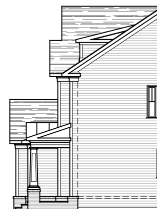
PARTIAL RIGHT ELEVATION ELEVATION #5B 06-02-25
