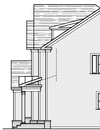
PARTIAL RIGHT ELEVATION ELEVATION #12A 06-02-25
