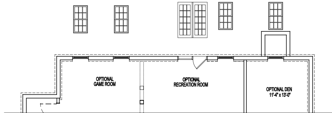
FOUNDATION / BASEMENT PLAN W/ WALKOUT
