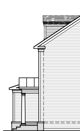
PARTIAL RIGHT ELEVATION ELEVATION #1A 06-02-25
