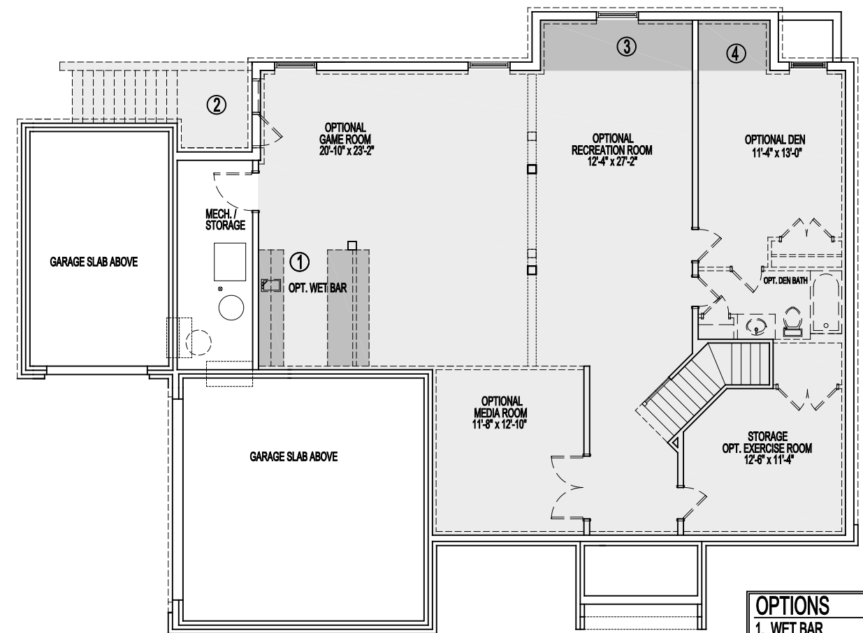
FOUNDATION / BASEMENT PLAN
