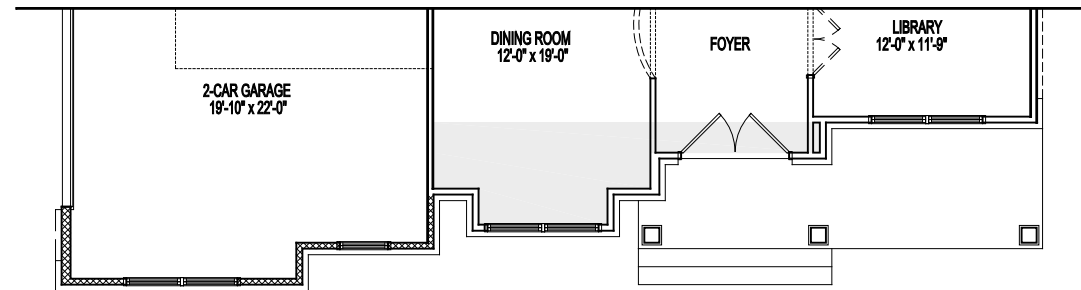
PARTIAL FIRST FLOOR PLAN ELEVATION #12B 06-02-25
