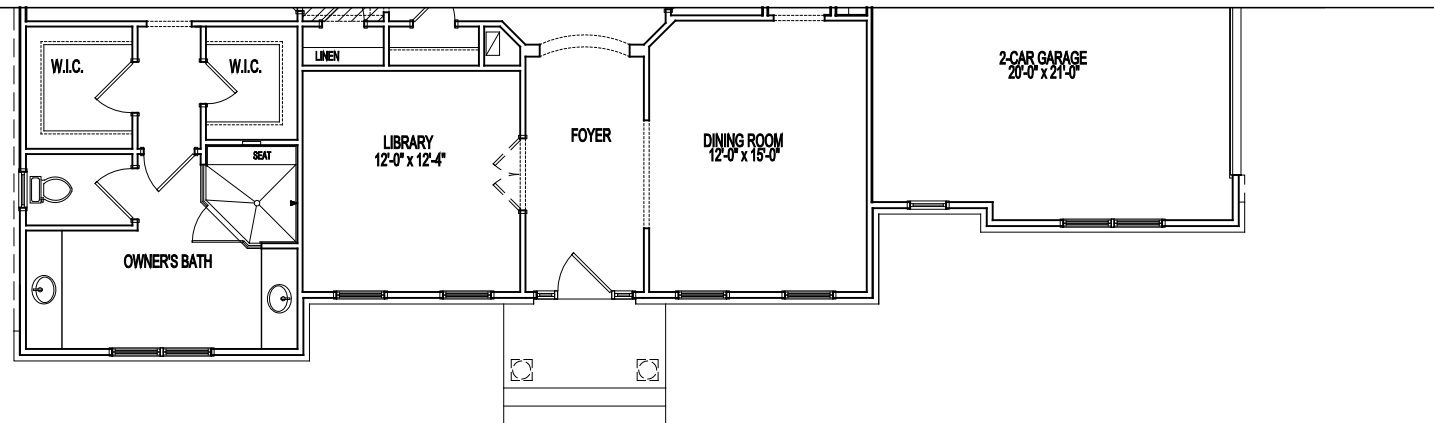
PARTIAL FIRST FLOOR PLAN
