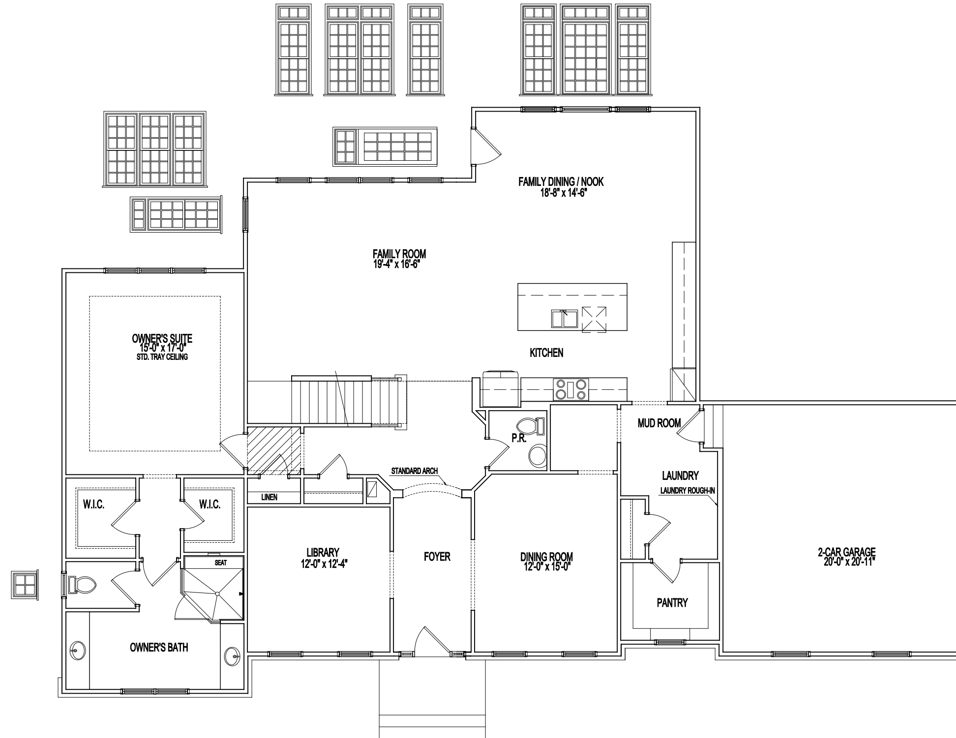
STANDARD FIRST FLOOR PLAN
