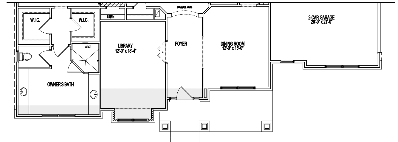
PARTIAL FIRST FLOOR PLAN ELEVATION 5B
