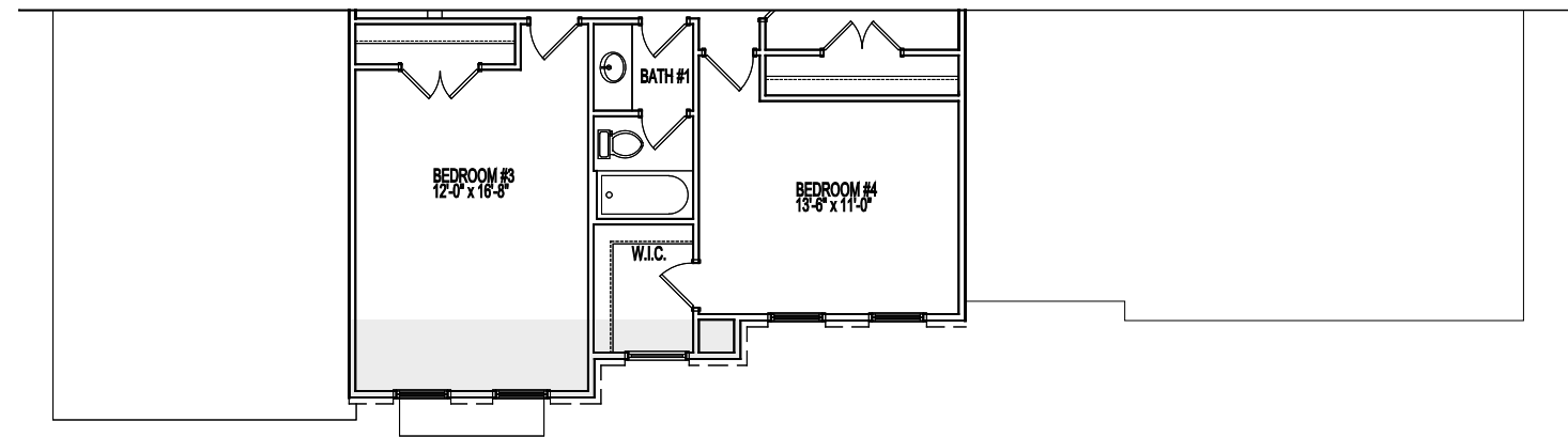
PARTIAL FIRST FLOOR PLAN ELEVATION 5B
