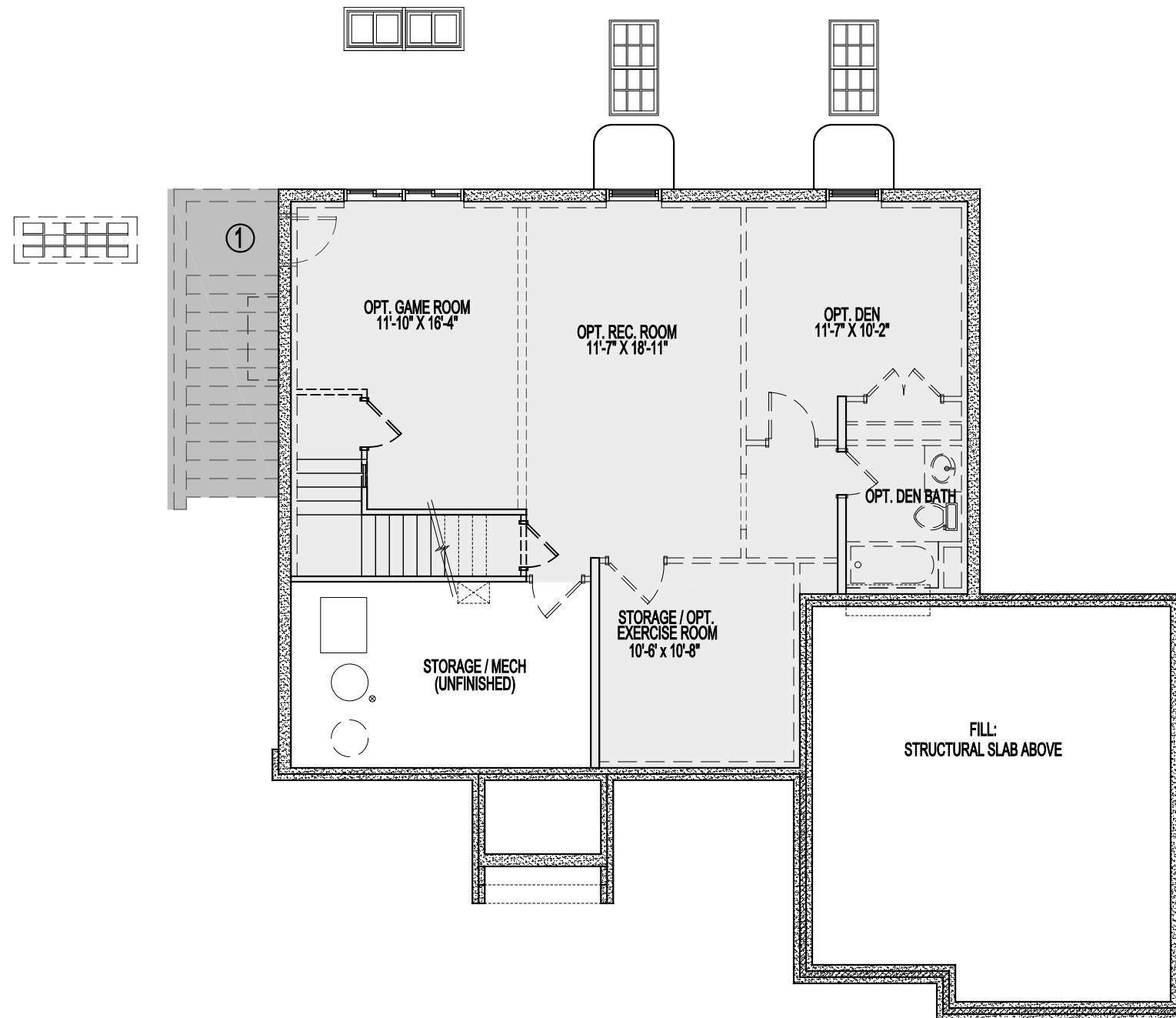
STANDARD FOUNDATION / BASEMENT PLAN STANDARD 8'-11" CEILING 02-07-2025
