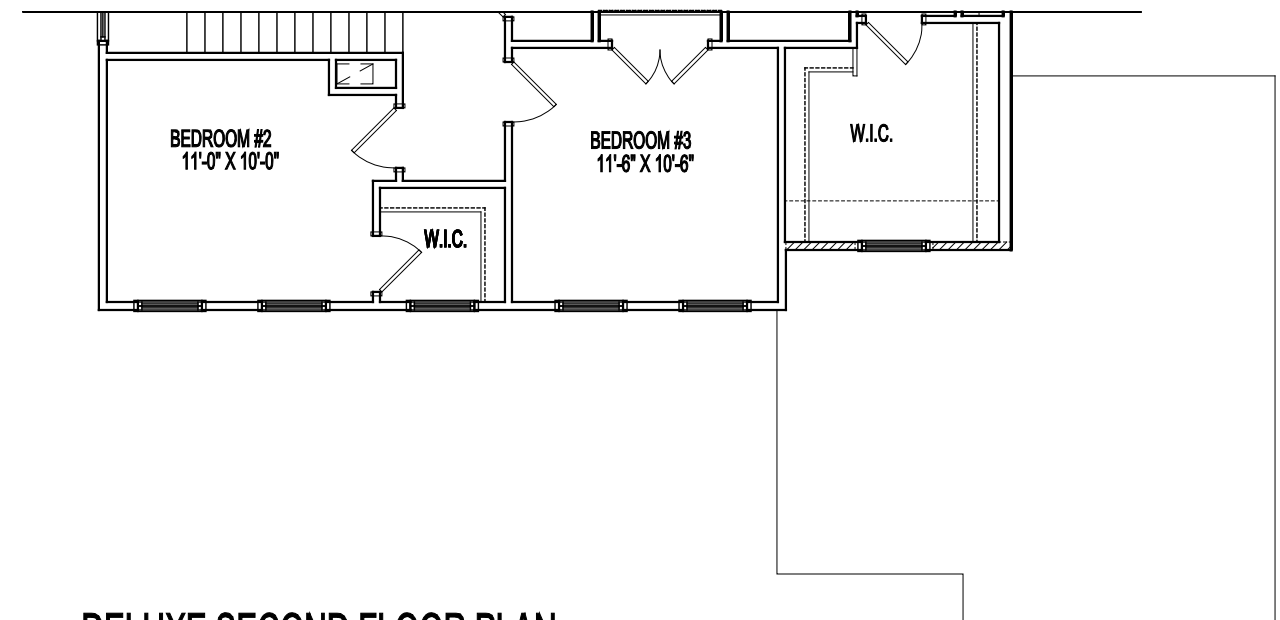
DELUXE SECOND FLOOR PLAN
