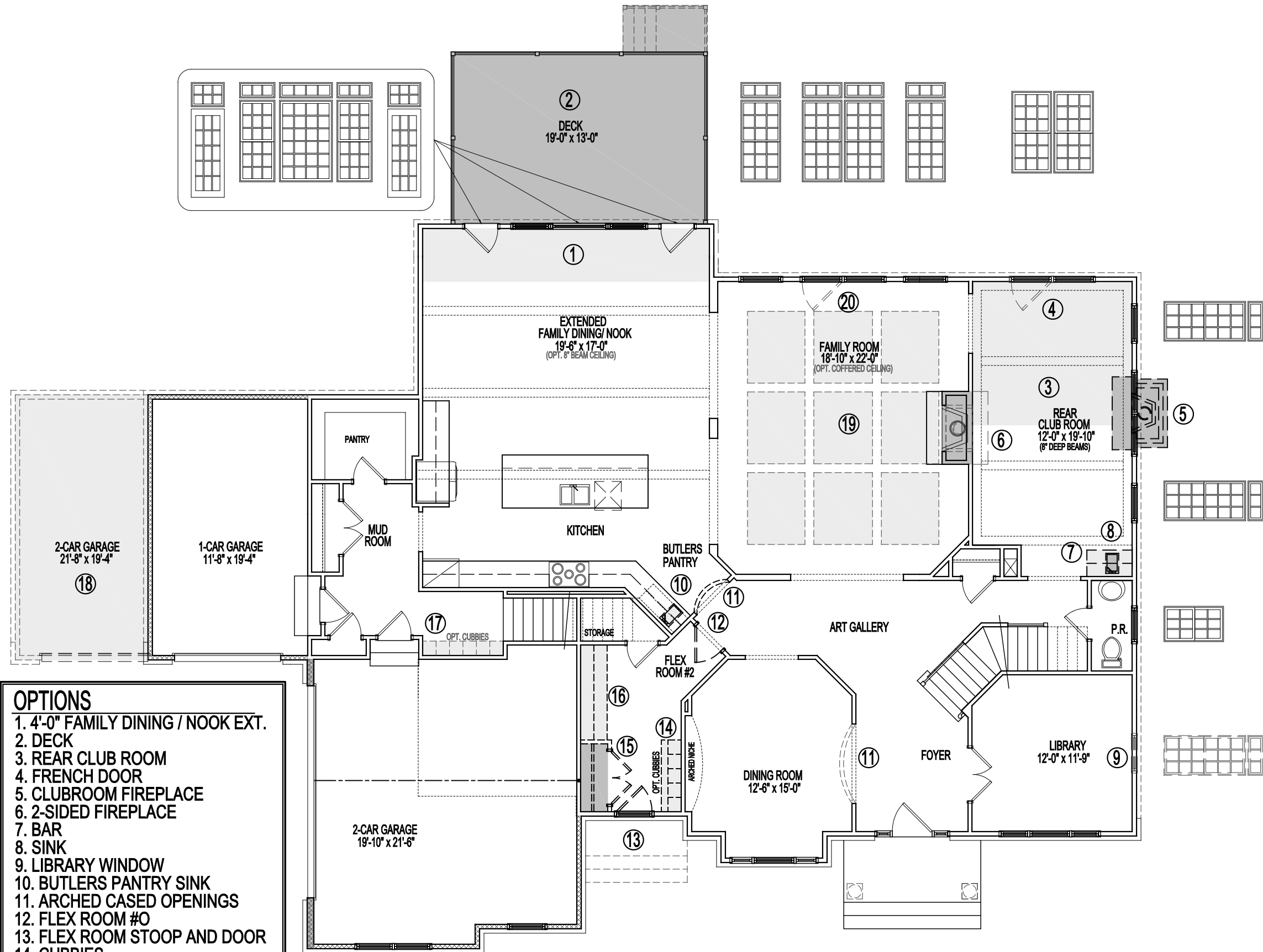
FIRST FLOOR PLAN 08-08-25
