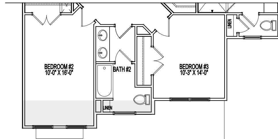
PARTIAL STANDARD SECOND FLOOR PLAN
