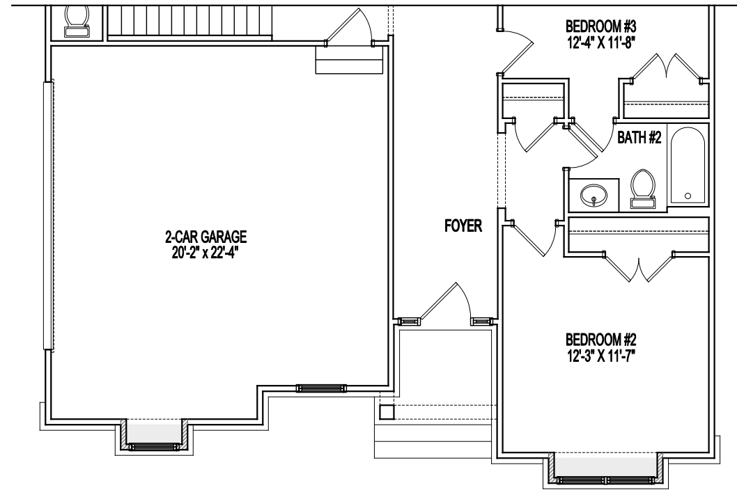
STANDARD FIRST FLOOR PLAN ELEVATION 2A STANDARD 9'-0" CEILING 07-16-2025
