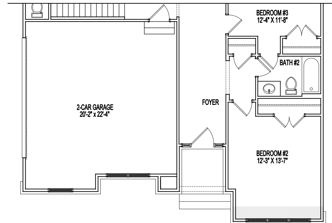
STANDARD FIRST FLOOR PLAN ELEVATION 5A STANDARD 9'-0" CEILING 07-16-2025
