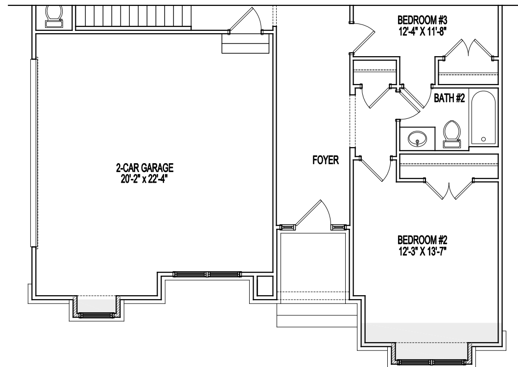
STANDARD FIRST FLOOR PLAN ELEVATION 4A STANDARD 9'-0" CEILING 07-16-2025
