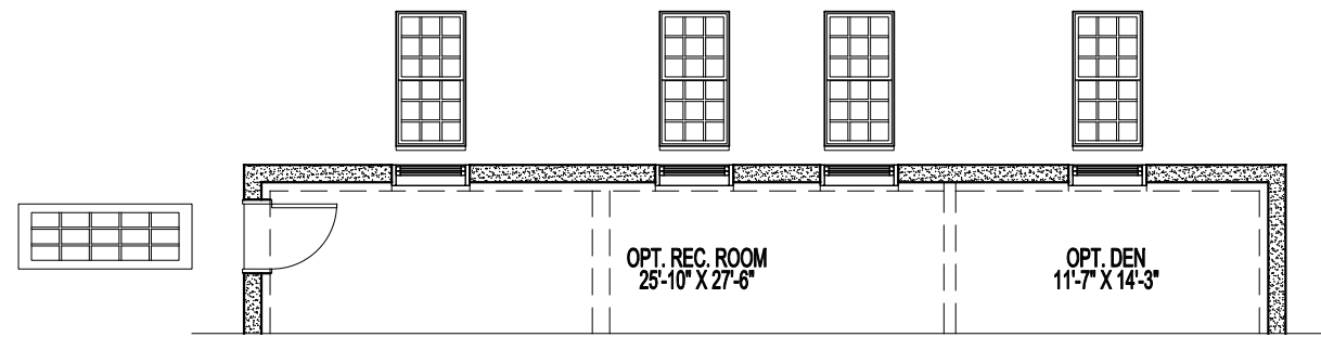
STANDARD FOUNDATION / BASEMENT PLAN STANDARD 8'-11\"/>
