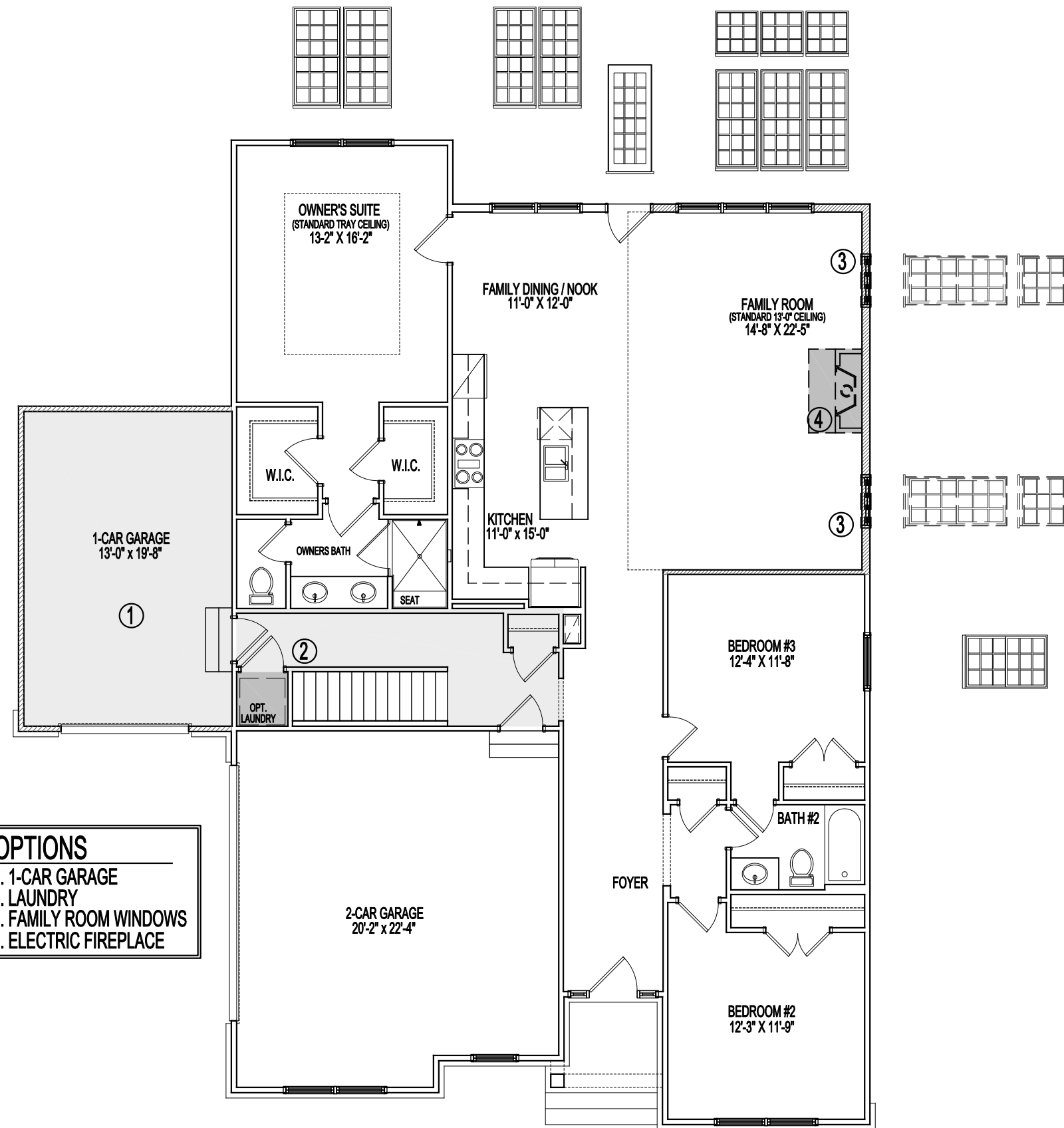
FIRST FLOOR PLAN STANDARD 9'-0" CEILING 07-16-2025
