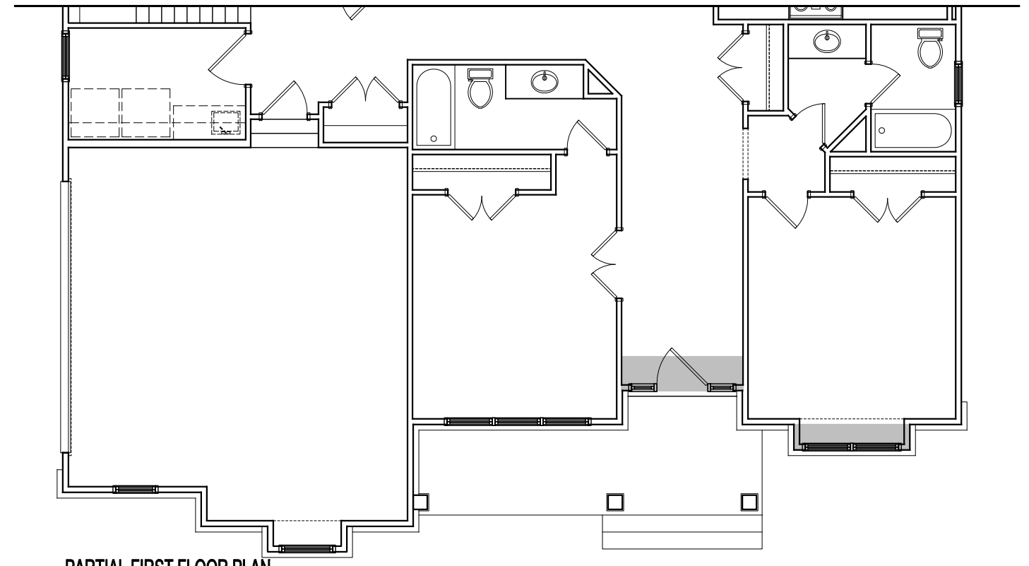
PARTIAL FIRST FLOOR PLAN
