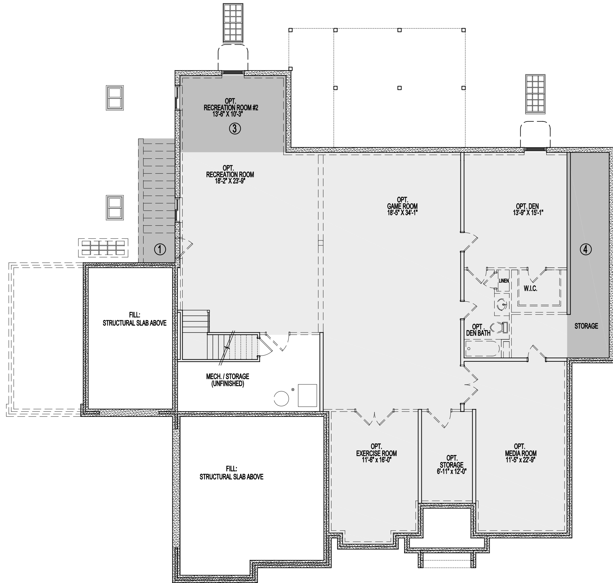
FOUNDATION PLAN STANDARD 8'-11" CEILING
