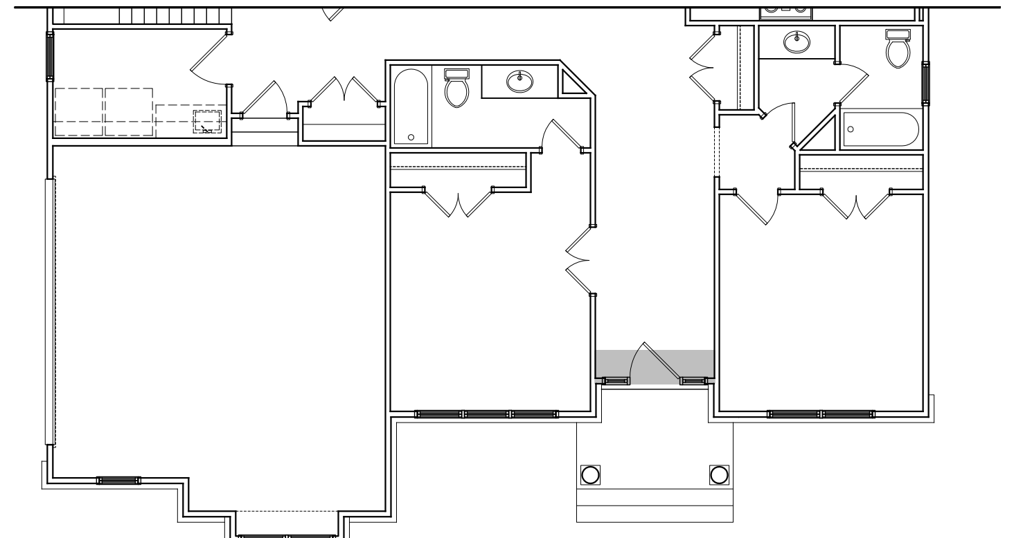
PARTIAL FIRST FLOOR PLAN
