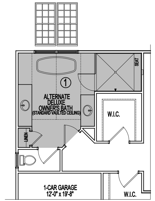
FIRST FLOOR PLAN STANDARD 10'-0" CEILING 03-14-2025
