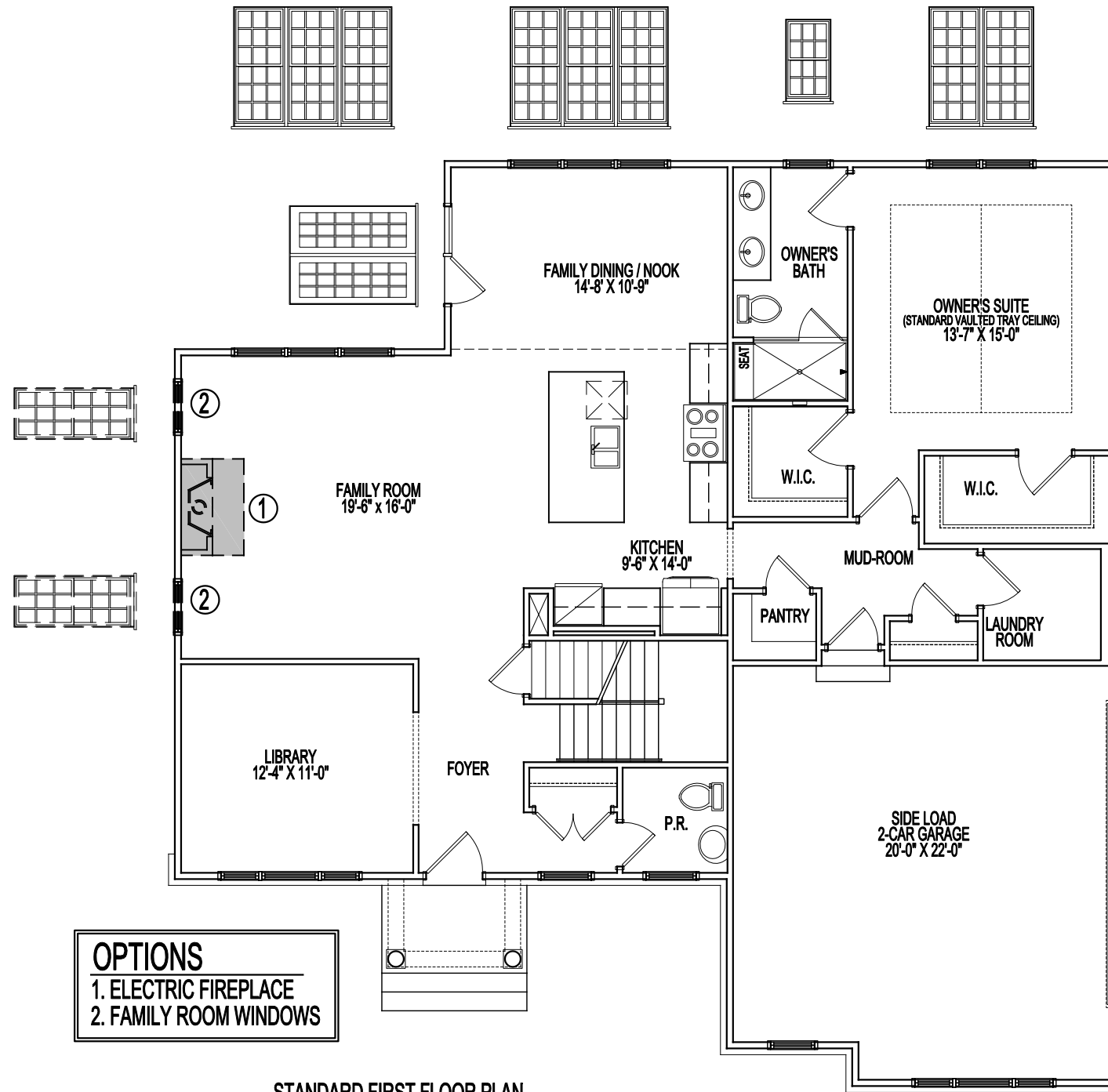
STANDARD FIRST FLOOR PLAN
