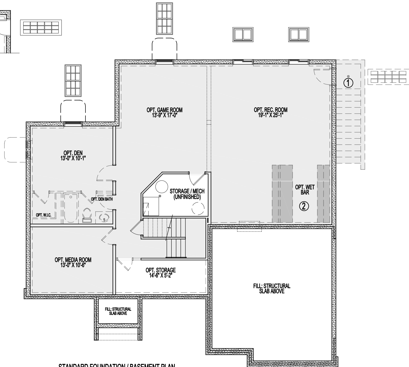
STANDARD FOUNDATION / BASEMENT PLAN STANDARD 8'-11" CEILING 01-22-2025
