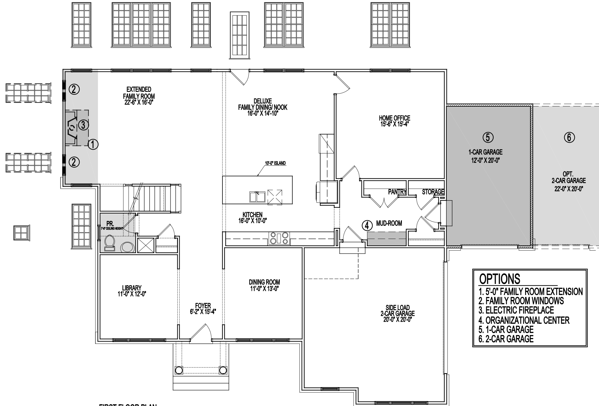
FIRST FLOOR PLAN STANDARD 9'-0" CEILING
