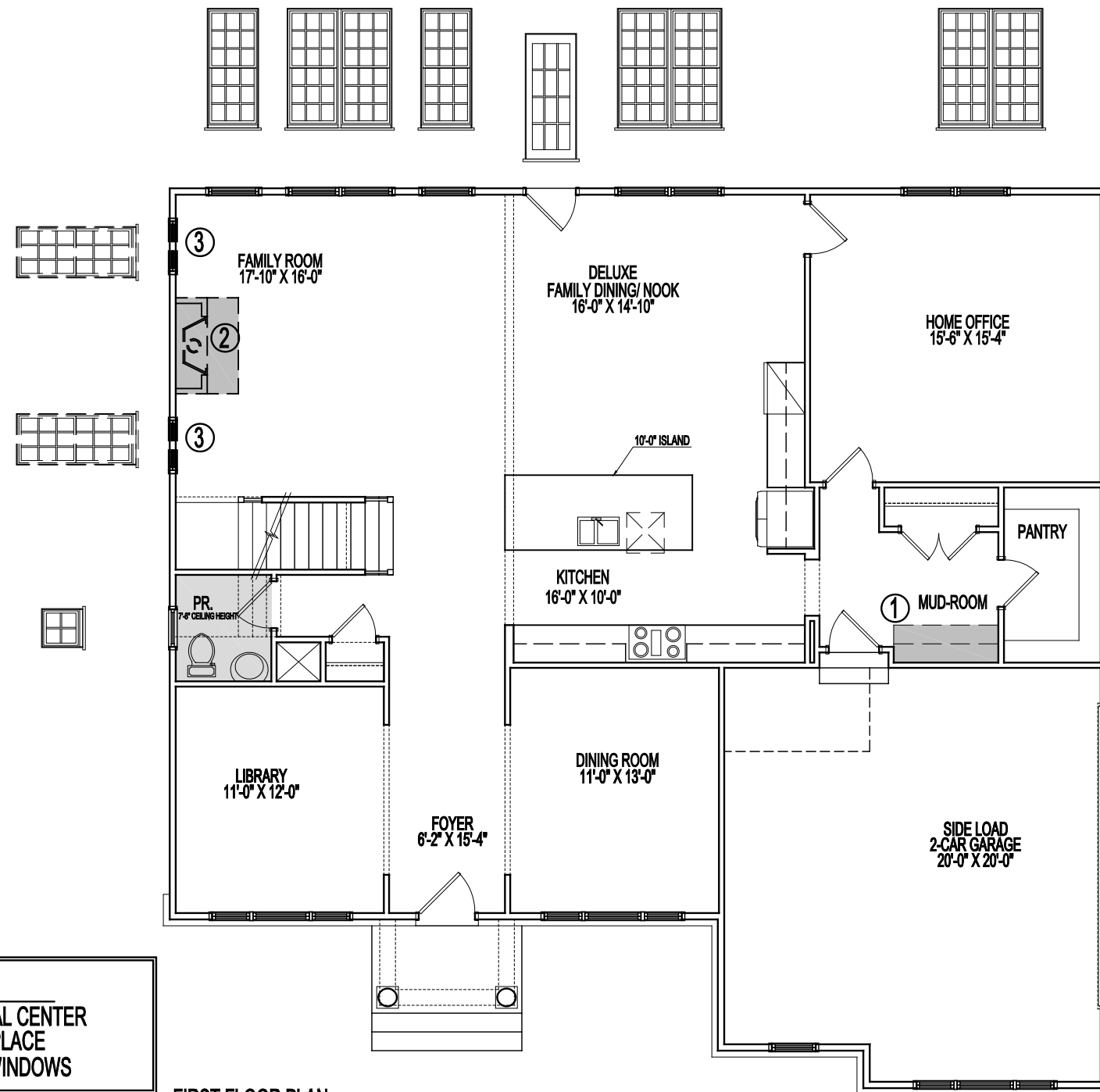
FIRST FLOOR PLAN STANDARD 9'-0" CEILING
