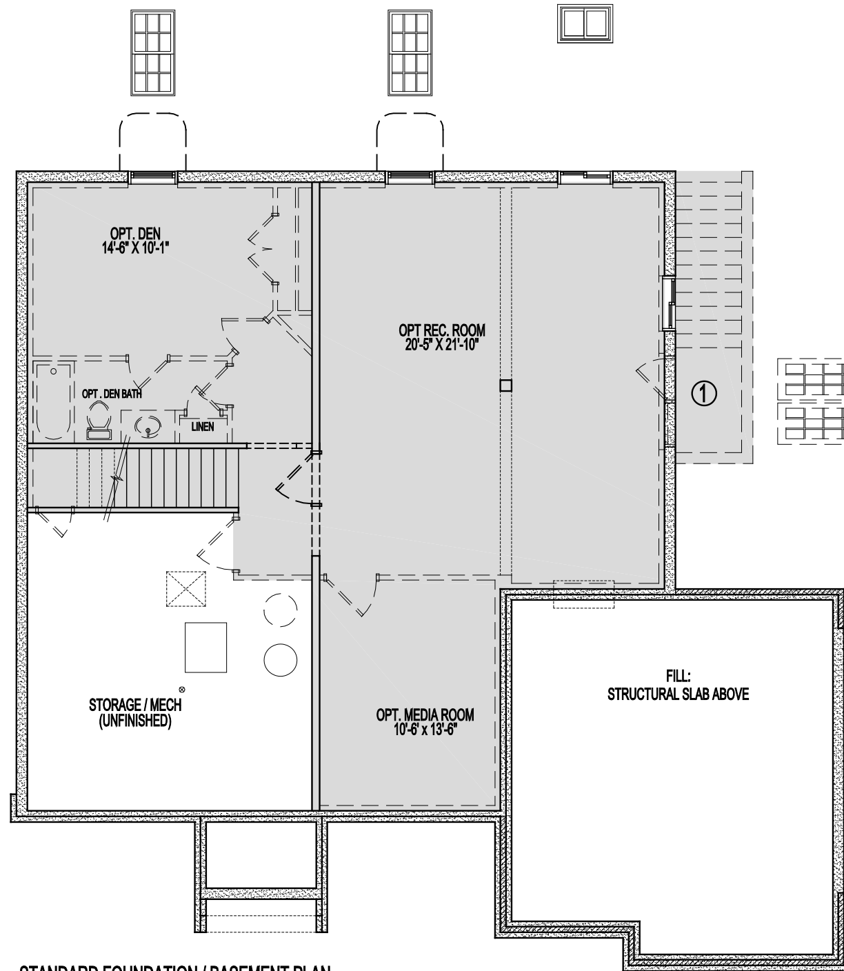
STANDARD FOUNDATION / BASEMENT PLAN STANDARD 8'-11" CEILING 01-24-2025
