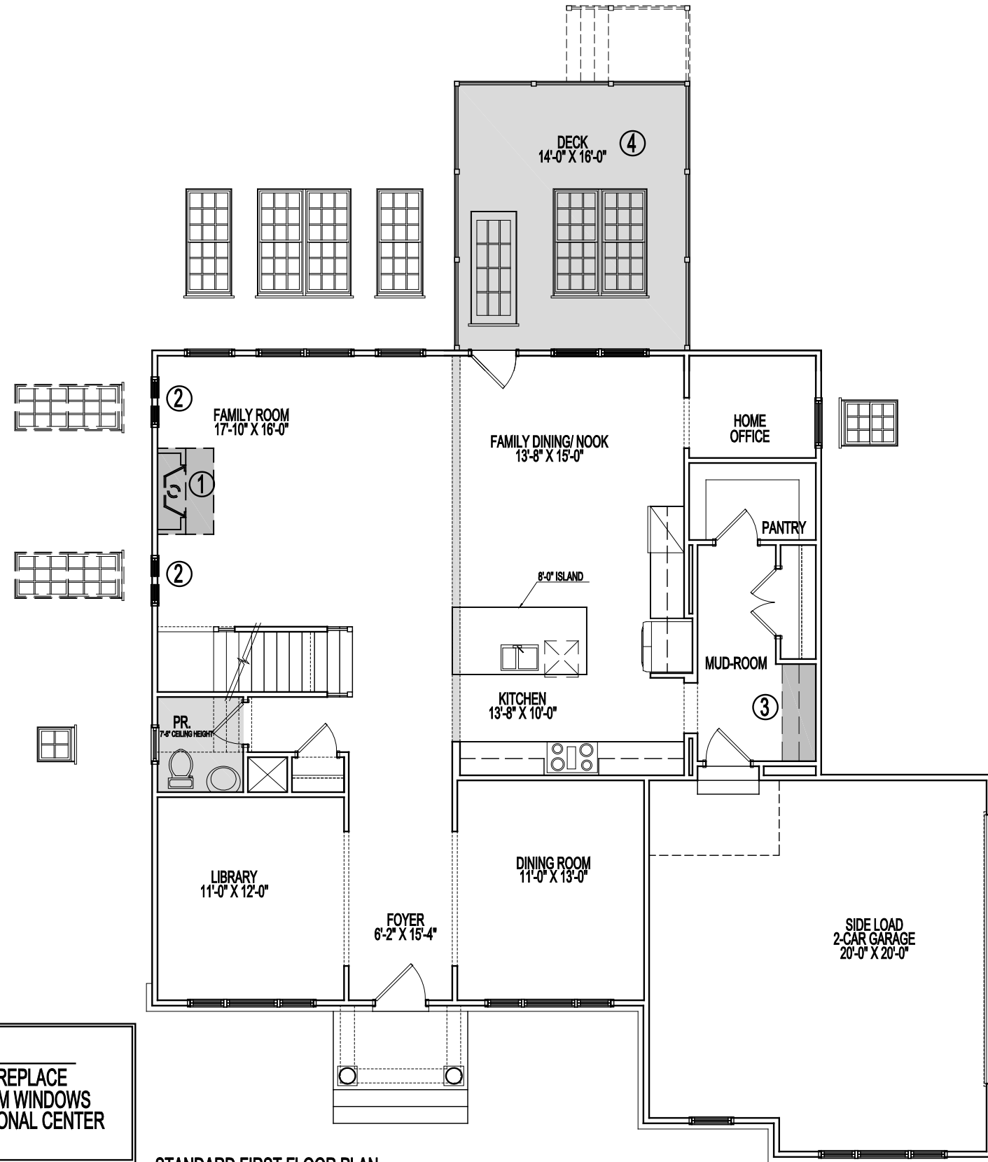
STANDARD FIRST FLOOR PLAN
