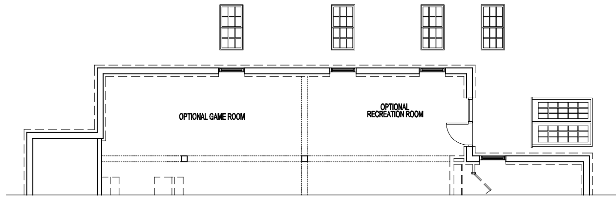
PARTIAL FOUNDATION / BASEMENT PLAN W/ WALKOUT 12-18-24 WINDOW LOCATIONS MAY VARY DUE TO GRADE
