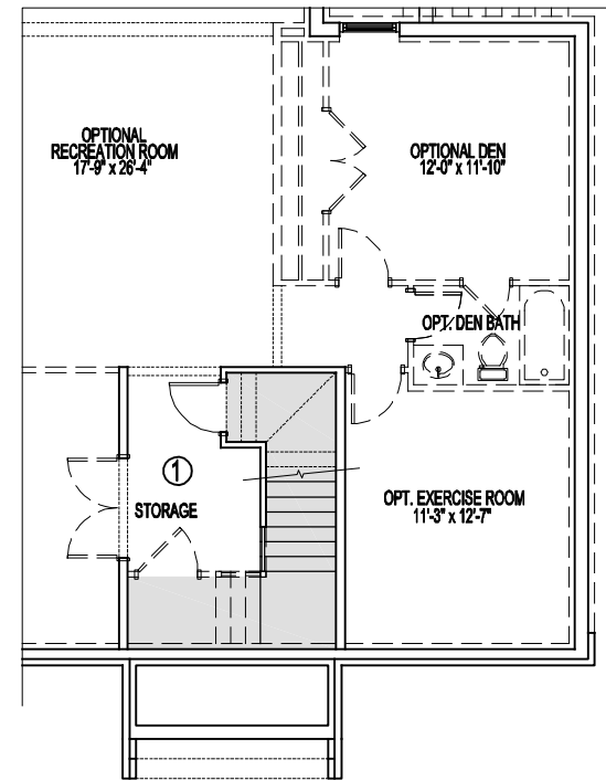
OPTIONS 1. STAIRS W/ 9'-11" CEILING HEIGHT PARTIAL BASEMENT PLAN 12-18-24
