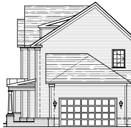
PARTIAL RIGHT SIDE ELEVATION ELEVATION #5B
