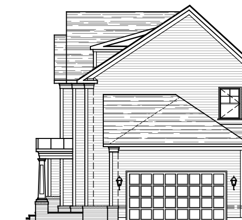
PARTIAL RIGHT SIDE ELEVATION ELEVATION #5A
