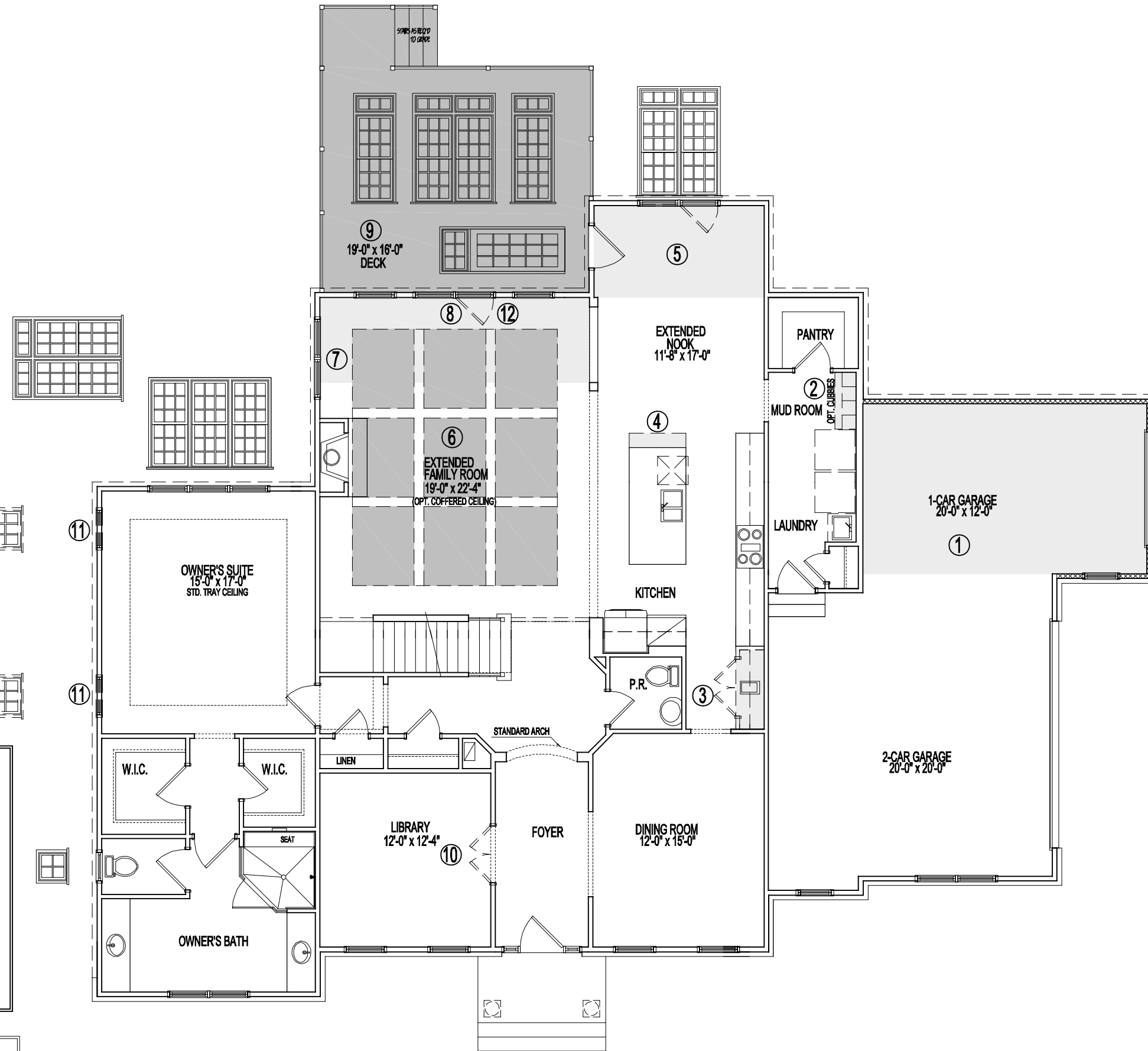
FIRST FLOOR PLAN 12-16-24
